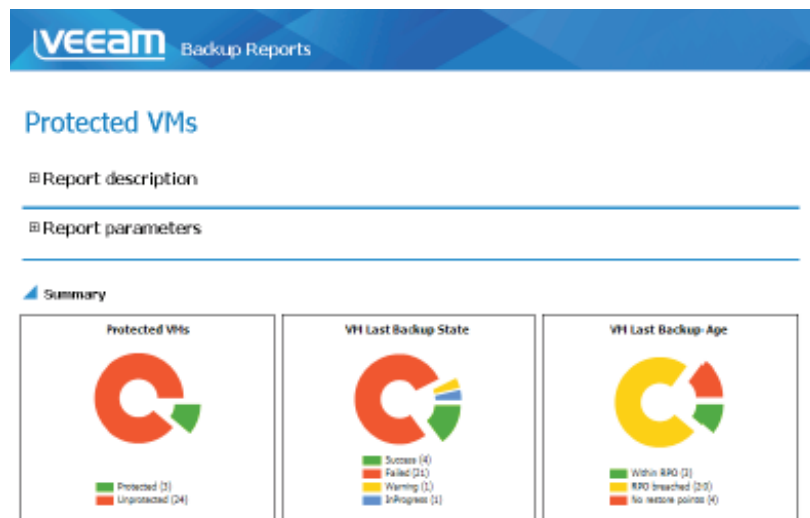
Figure 2. The protected VMs report analyzes backup protection of your VMs
